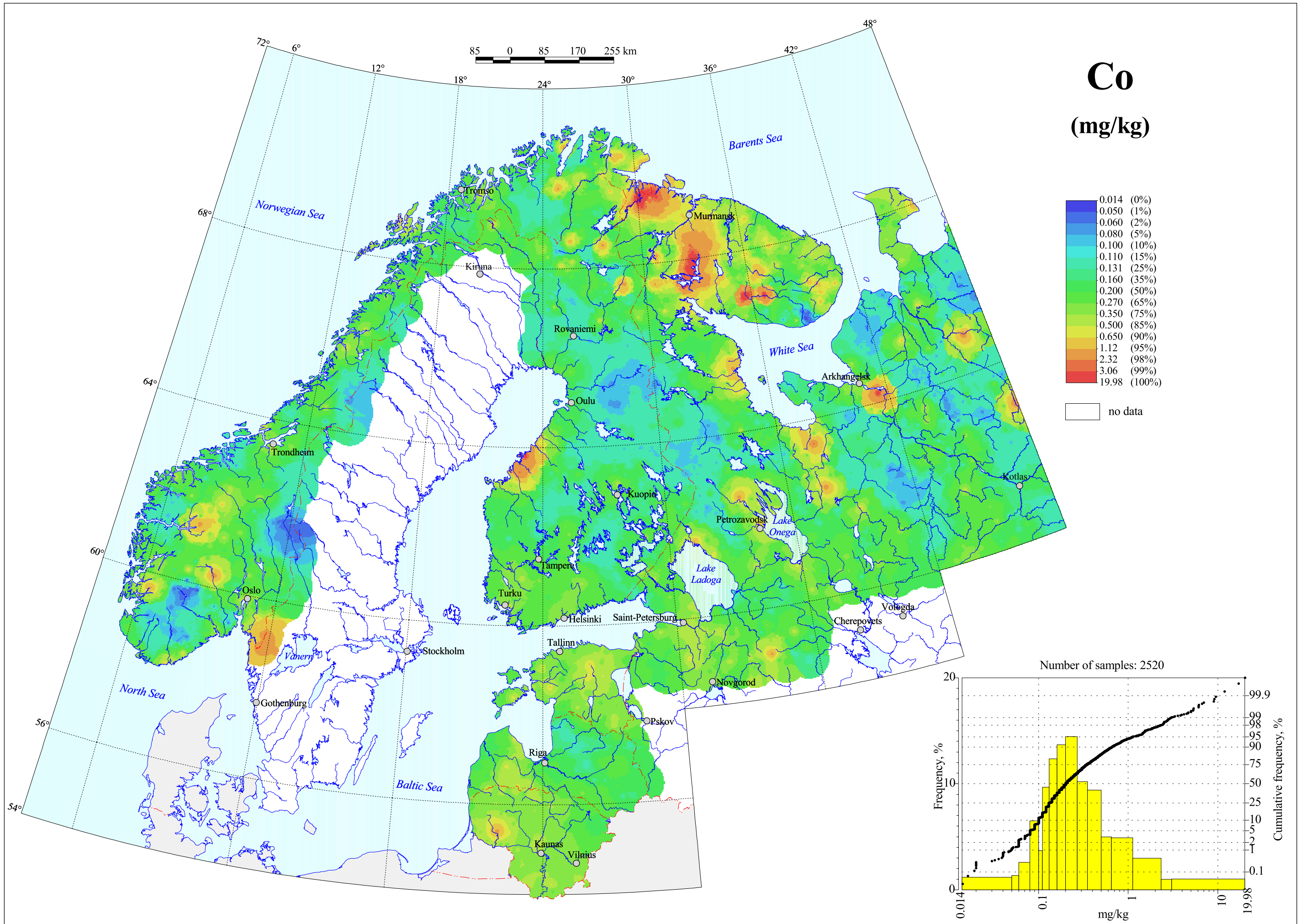
Cobalt in Terrestrial Moss, Total Content
